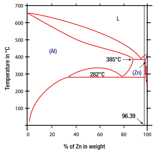
Zinc aluminium diagram
